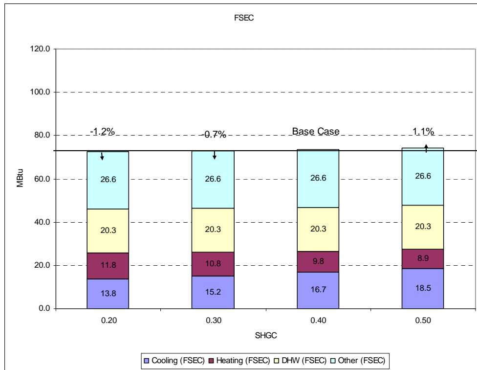
Figure 38. SHGC (FSEC) without the duct leakage.
