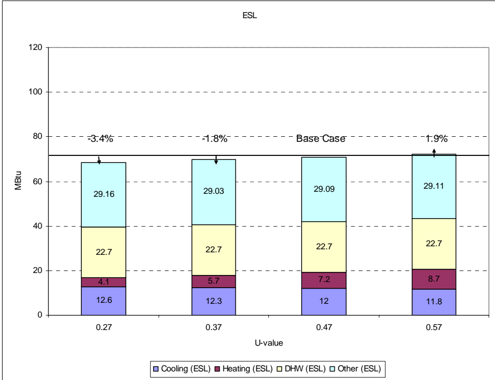
Figure 39. U-value (ESL) without the duct leakage.
