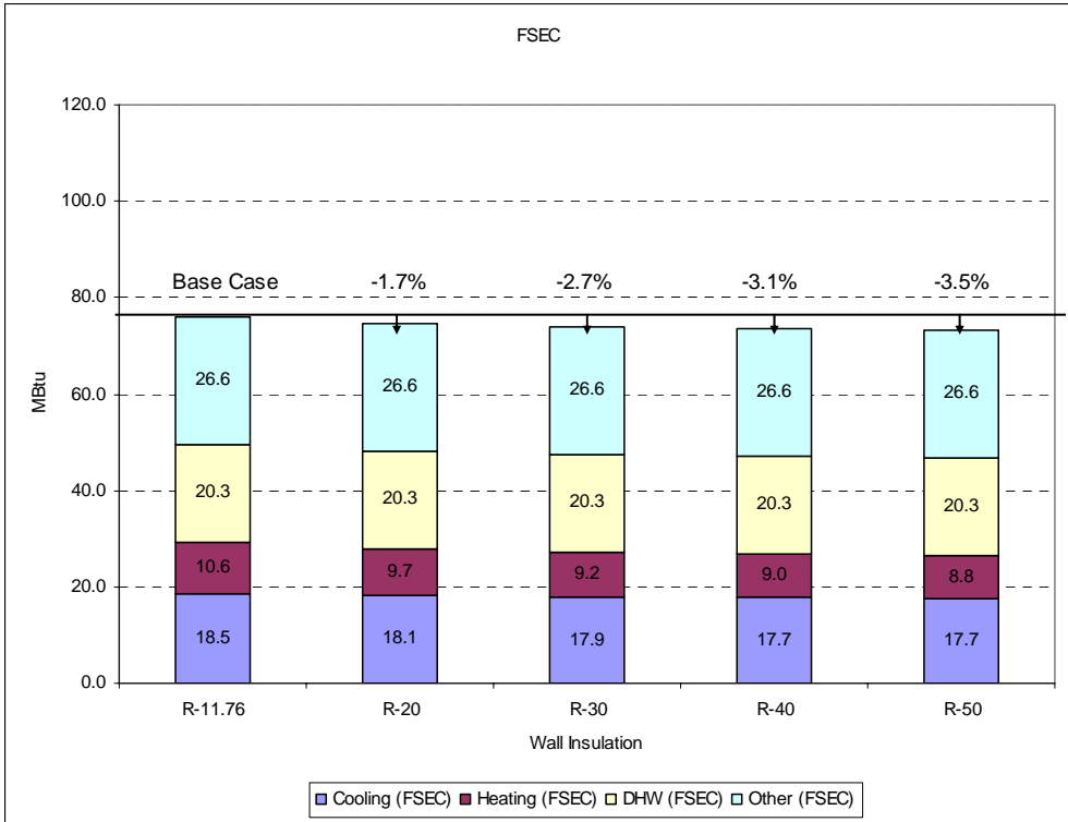
Figure 10. Wall insulation (FSEC) with the duct leakage.
