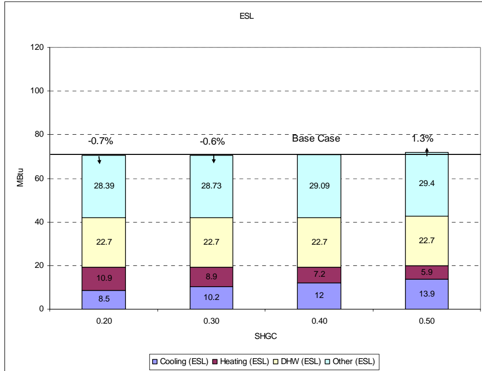
Figure 37. SHGC (ESL) without the duct leakage.
