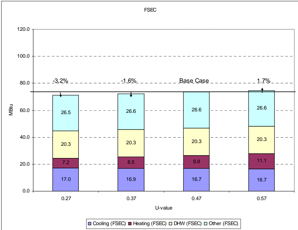
Figure 40. U-value (FSEC) without the duct leakage.
