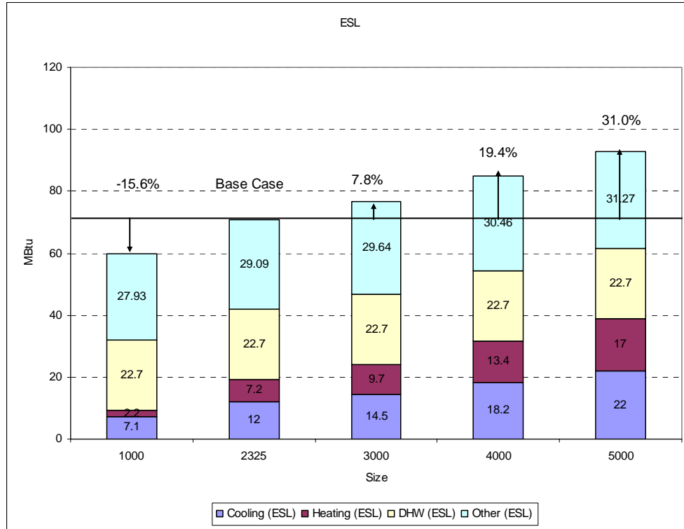
Figure 43. Size (ESL) without the duct leakage.
