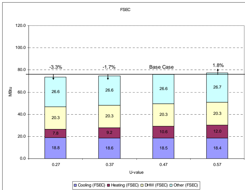
Figure 18. U-value (FSEC) with the duct leakage.
