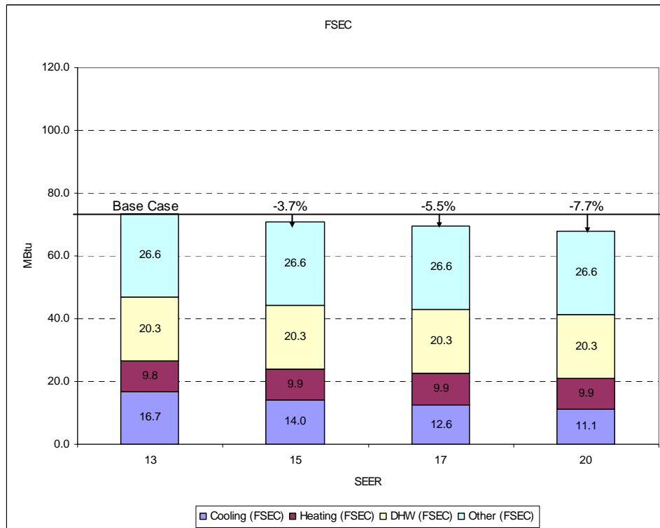
Figure 26. SEER (FSEC) without the duct leakage.
