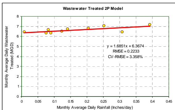
Fig. 4. Monthly average daily wastewater treated versus rainfall
