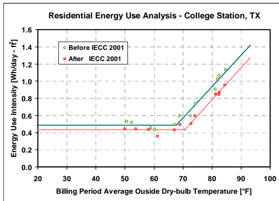
Figure 5. Comparison of energy use intensity from the implementation of the IECC 2000/2001 for the period of July 2003 through June 2004.
