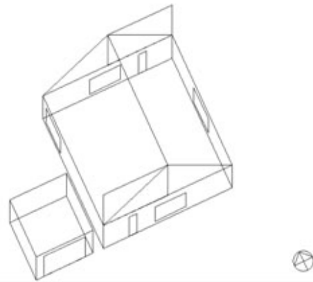
Figure 2: DrawBDL (Huang & Associates 2000) View of Base-case Model.
