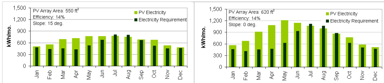
Figure 6. Sizing of Photovoltaic System in Houston (Left) and Phoenix (Right)
